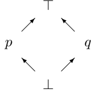
Figure 1: Lattice L
